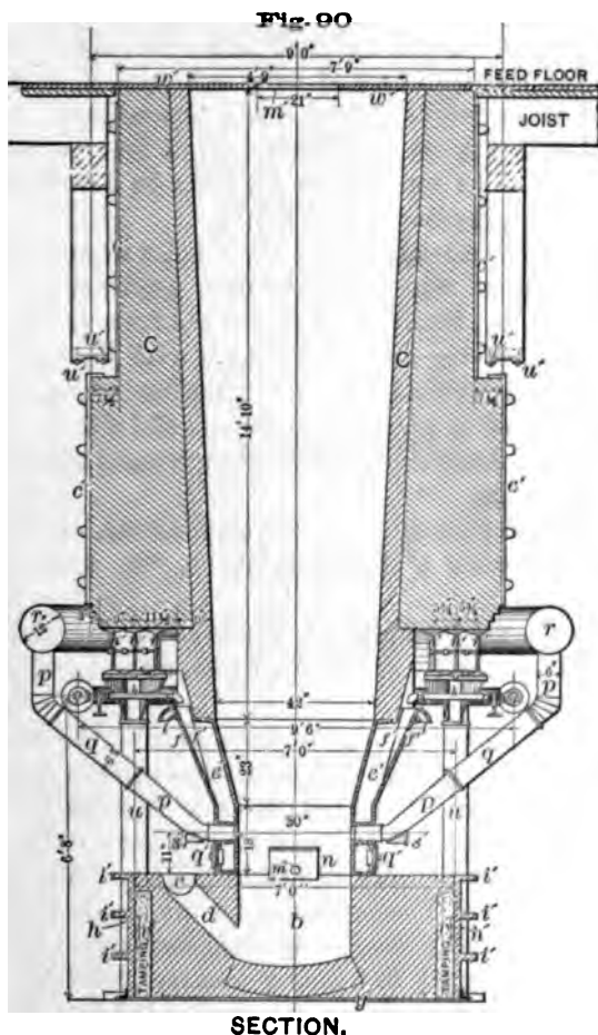
BLAST-FURNACE OF THE GLOBE SMELTING CO.'S WORKS, DENVER, COL.
